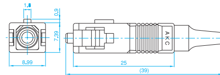
Fiber Jacket Φ0.9mm
