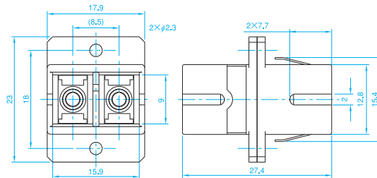
Adapter (SCH-2A)
