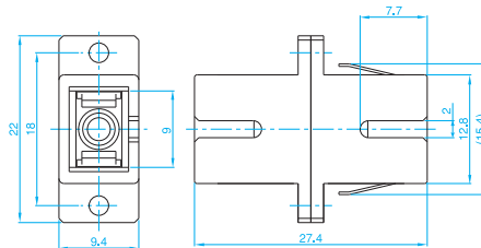
Adapter
