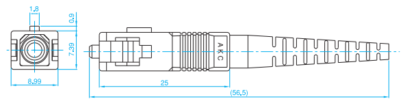
Fiber Cable \Phi 2.0\text{mm}
